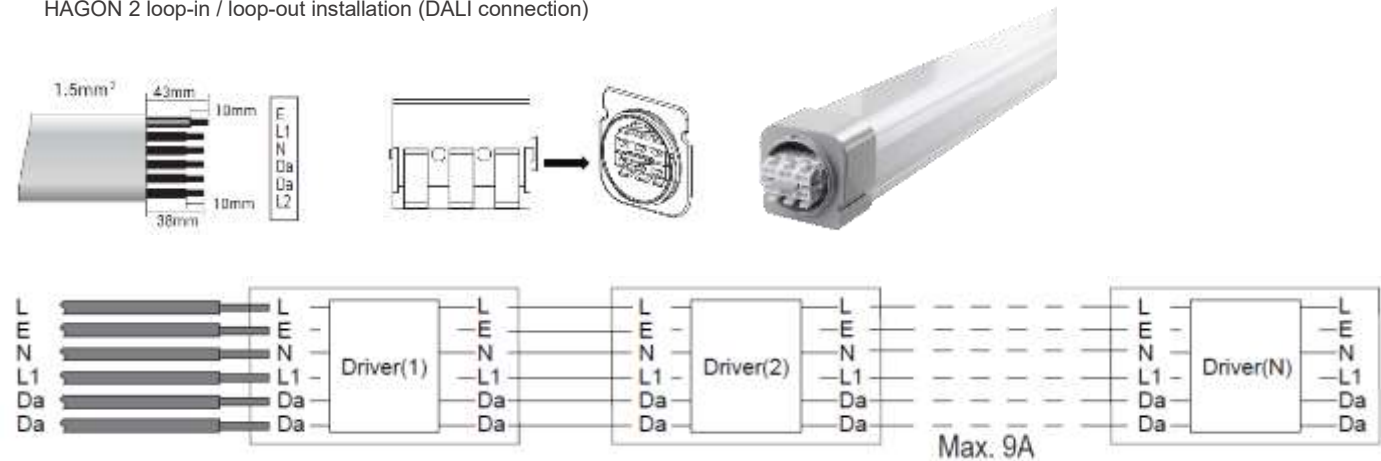
HAGON 2 loop-in / loop-out installation (DALI connection)
